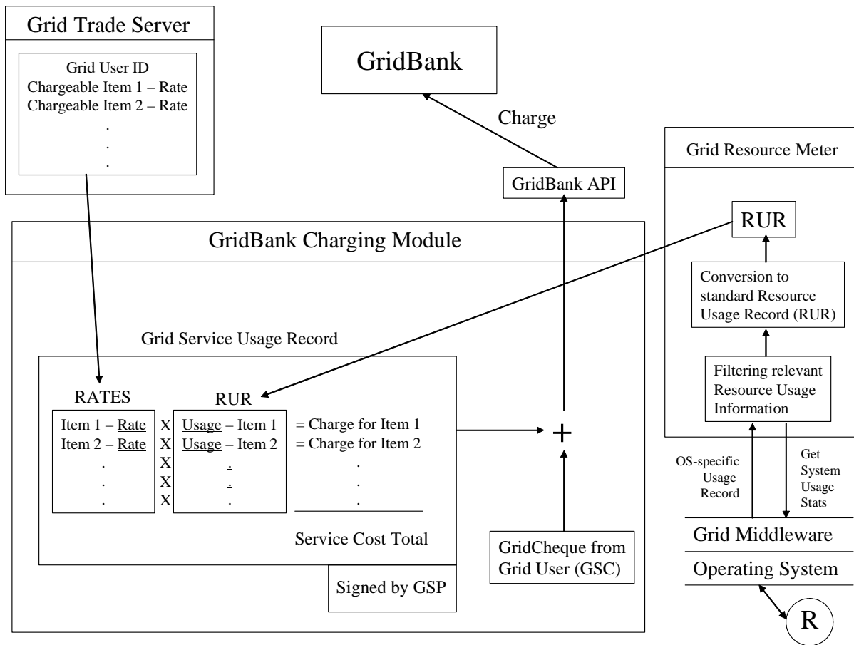
Figure 2: Interaction between the GTS, GBCM, GRM and GridBank.
