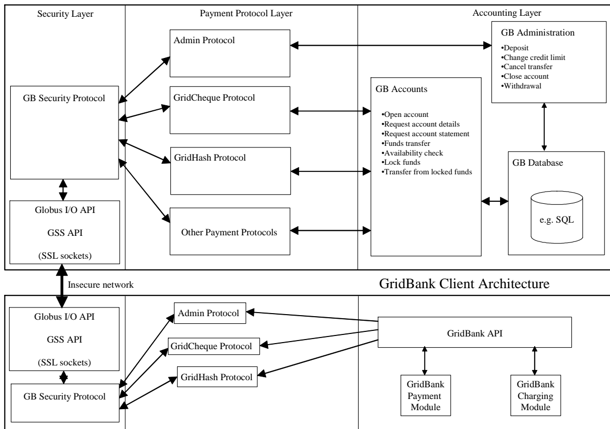
Figure 3: GridBank Server Architecture.
