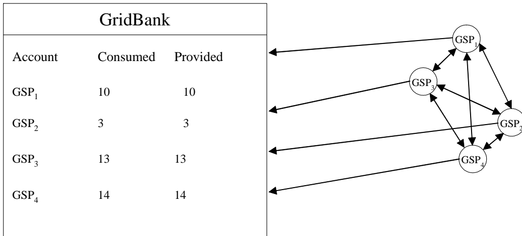
Figure 4: Co-operative Resource Sharing.
